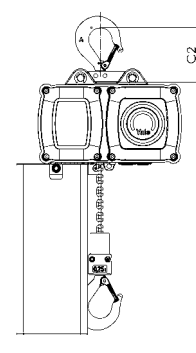
CPV/CPVF with suspension lug, 250 - 2500 kg
